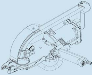
F CL45A Gabion Tool
